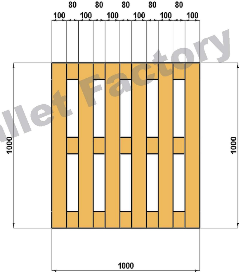
Bottom View
